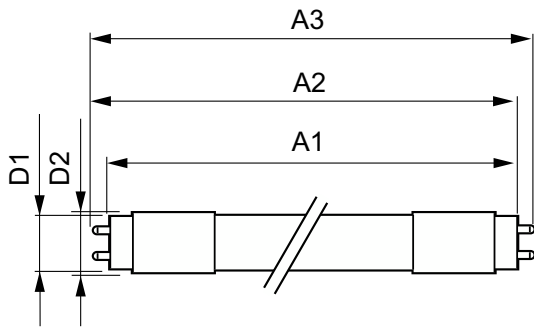
MASTER LEDtube STD 1200mm 10.5W865 T8
