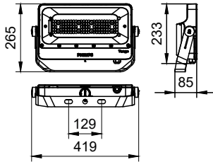
BVP431 LED68/NW 220~240V 50W SMB GC
