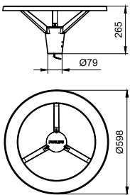
BGP161 LED2300/WW PSU 220-240V 9006 IN
