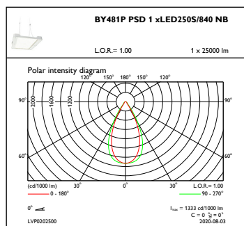
OFPC1_BY481PPSD1xLED250S840NB
